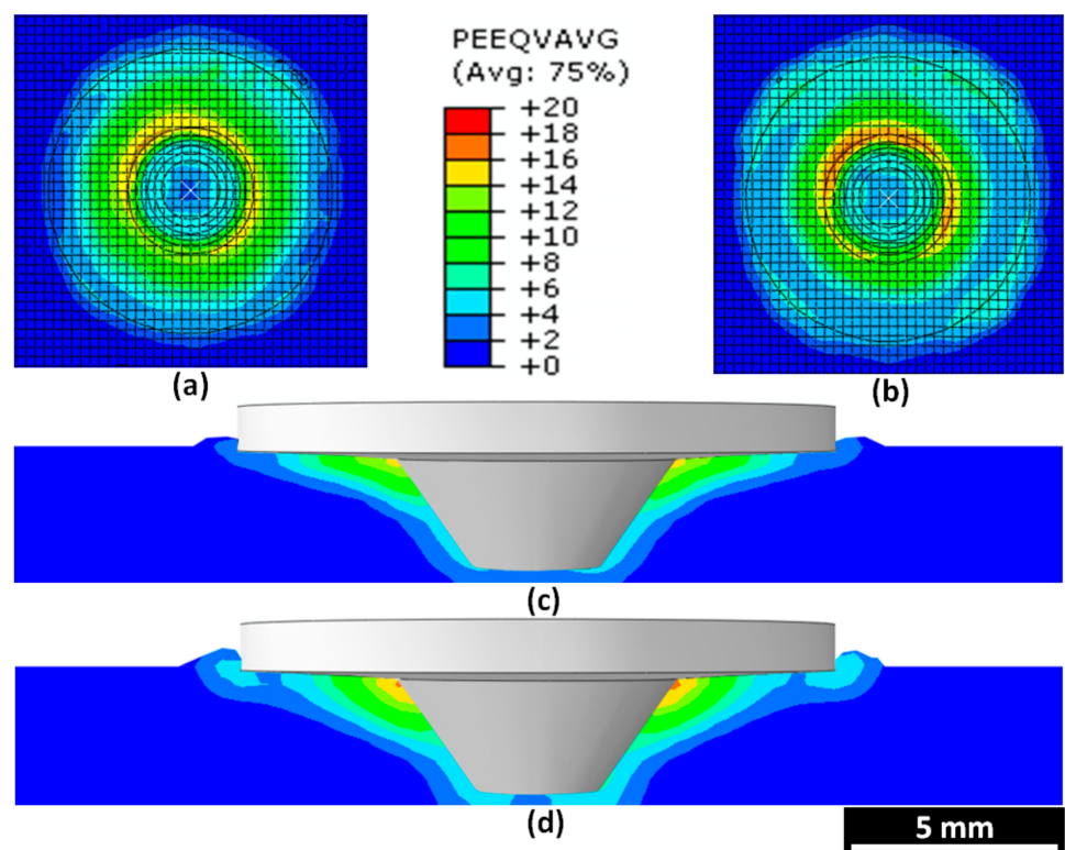
Figure 6. Equivalent plastic strain distribution at plunge and dwell stages. (a) Top view at plunge, (b) top view at dwell, (c) cross section view at plunge, and (d) cross section view at dwell.
